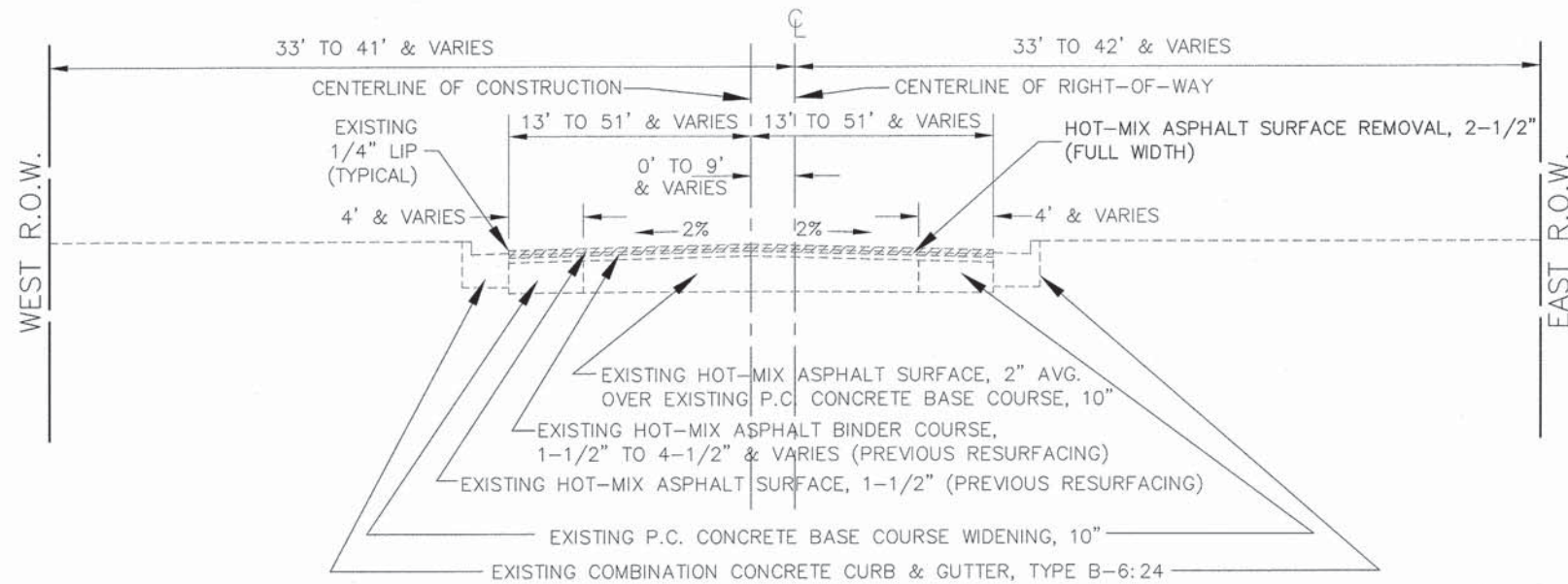
EXISTING TYPICAL SECTION STA. 27+50 TO STA. 39+89, LAWNDALE AVENUE
