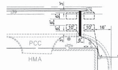
DETECTOR LOOP INSTALLATION AT 47TH STREET
