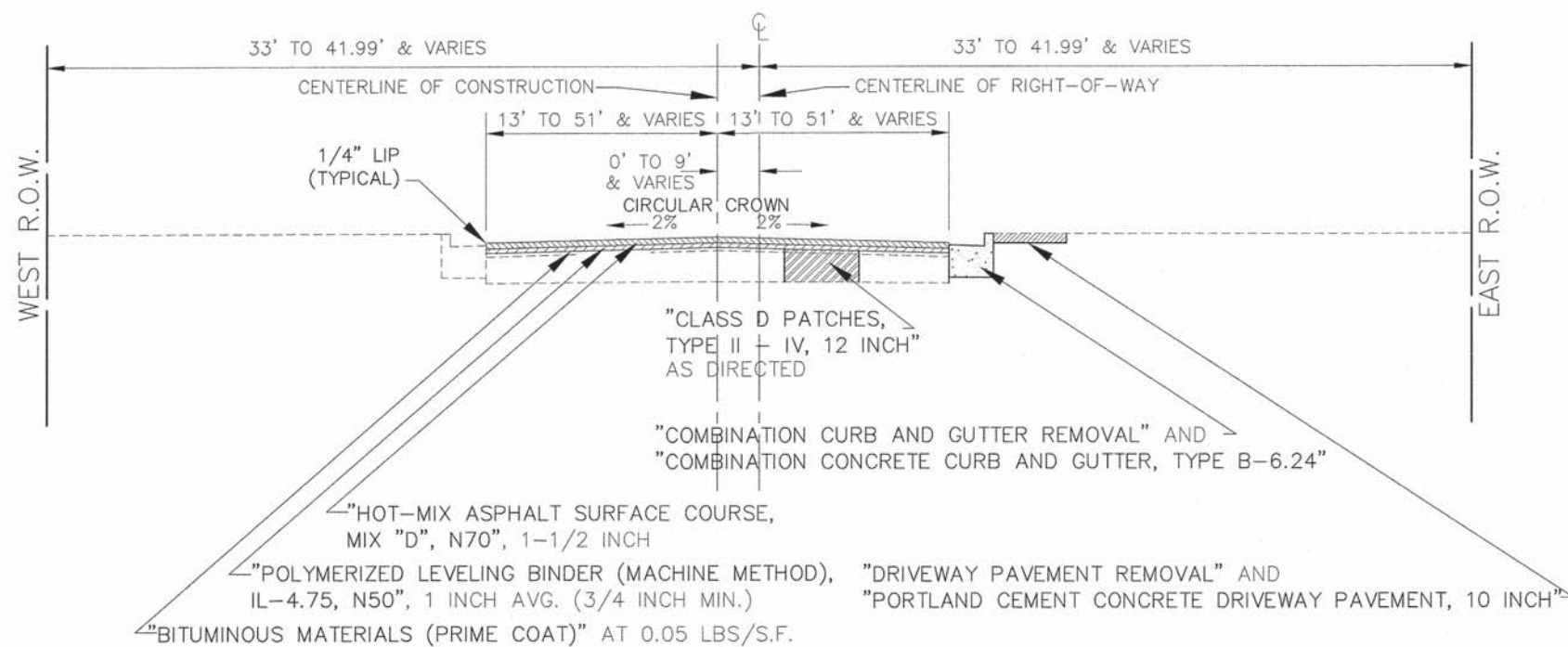
PROPOSED TYPICAL SECTION STA. 27+50 TO STA. 39+89, LAWNDALE AVENUE
