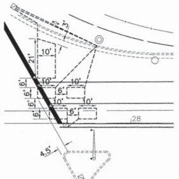
DETECTOR LOOP INSTALLATION AT JOLIET ROAD
