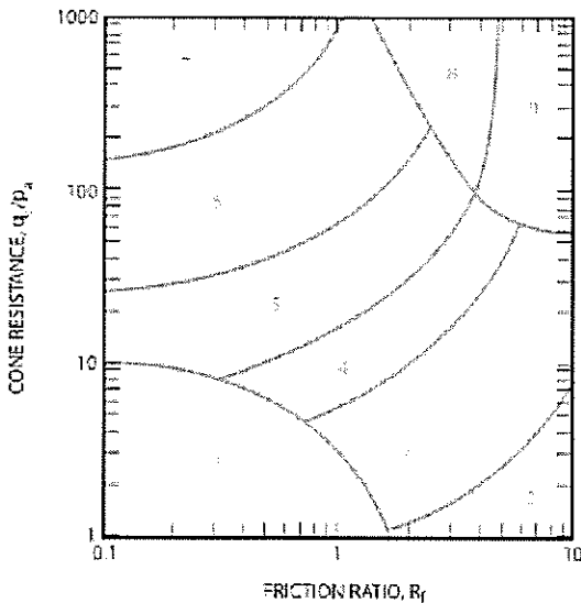
Non-normalized CPT Soil Behavior Type (SBT) chart
