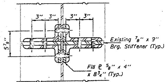
SECTION L-L
