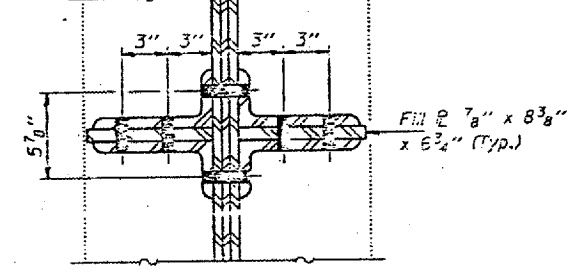
SECTION O-O
