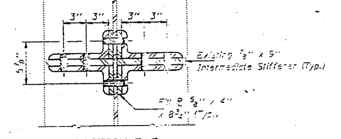
SECTION P-P
