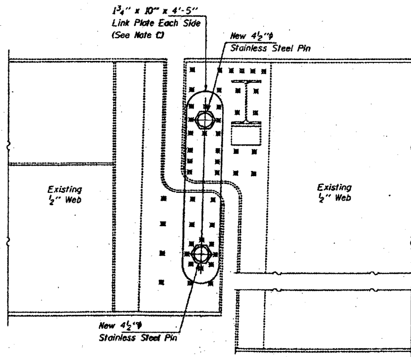
ELEVATION AT NEW PIN ASSEMBLY SPAN 4
