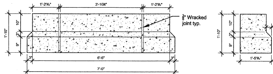
D Precast Cap 3 d-precast panel C 3/4" = 1'-0"
