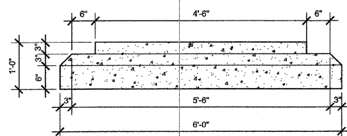
B Precast Cap 1 d-precast cap A 3/4" = 1'-0"
