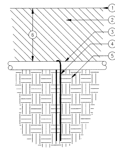
TYPICAL 0.5 GPH IRRIGATION BED LAYOUT
