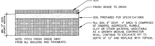
SOD DETAIL NOT TO SCALE
