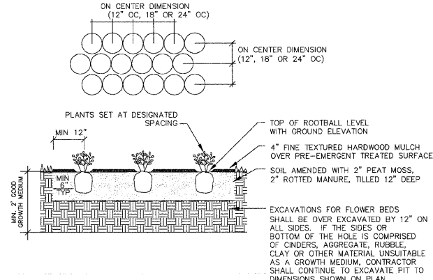
PERENNIAL PLANTING DETAIL NOT TO SCALE
