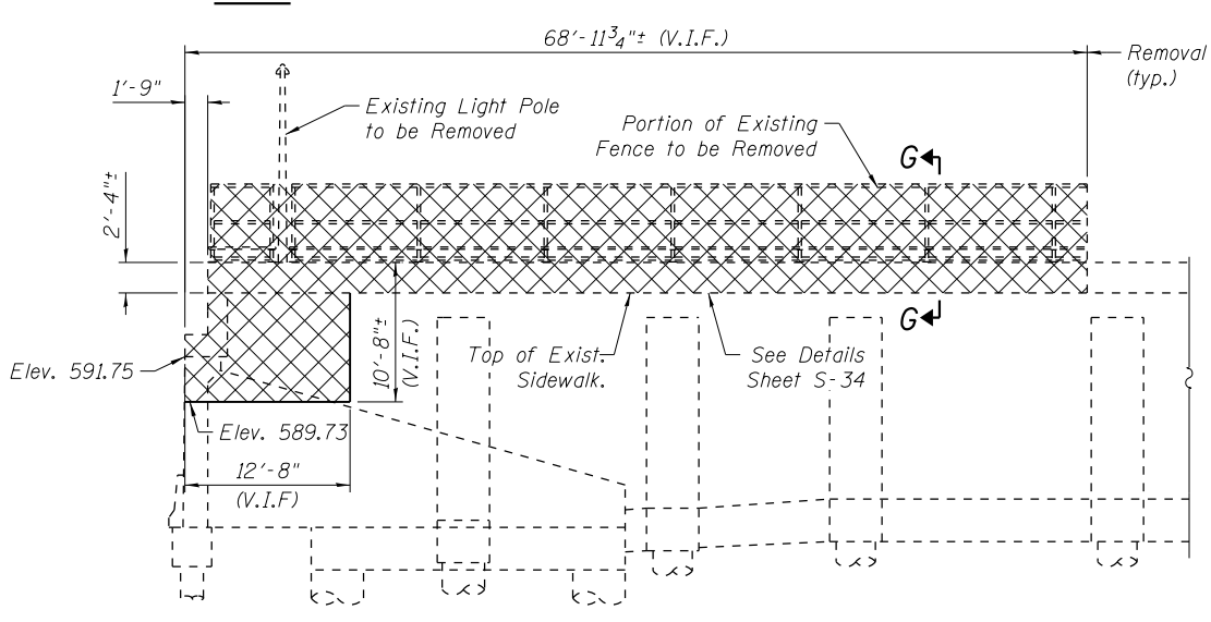
SECTION E-E
