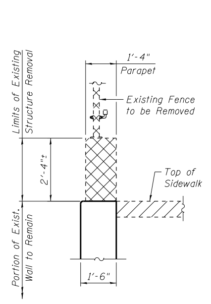
SECTION G-G
