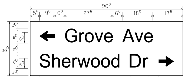
PANEL SIGN DESIGN TYPE 2
