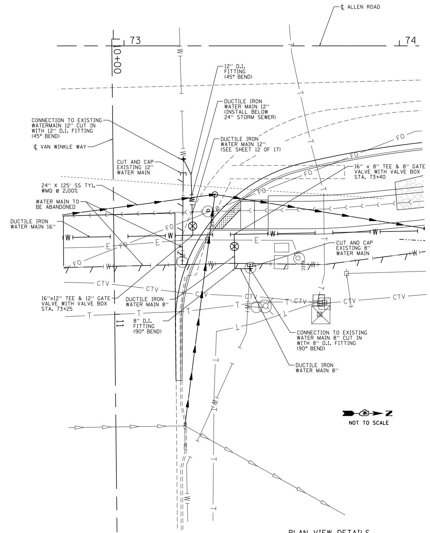
PLAN VIEW DETAILS VAN WINKLE WAY
