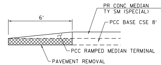
PCC RAMPED MEDIAN TERMINAL
