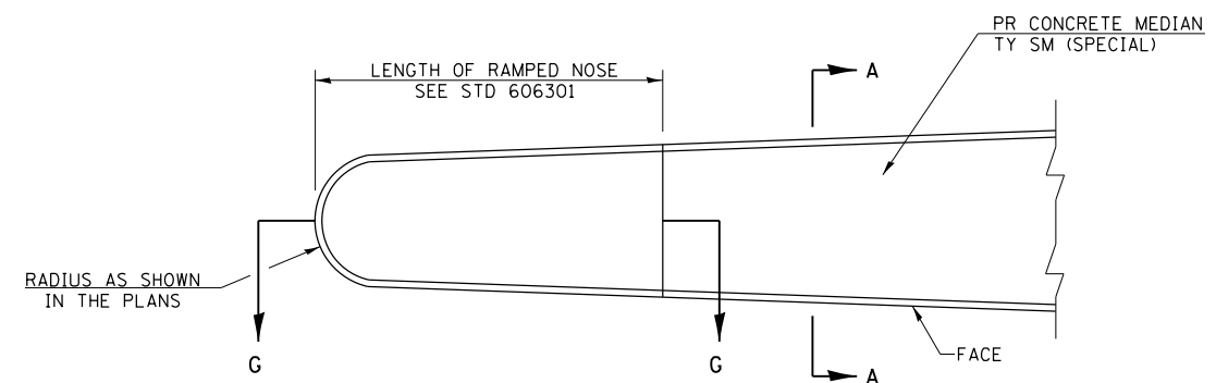
PLAN OF CONCRETE MEDIAN TY SM (SPECIAL)
