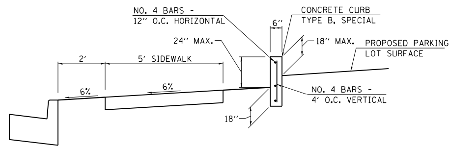
CONCRETE CURB TYPE B, SPECIAL DETAIL
