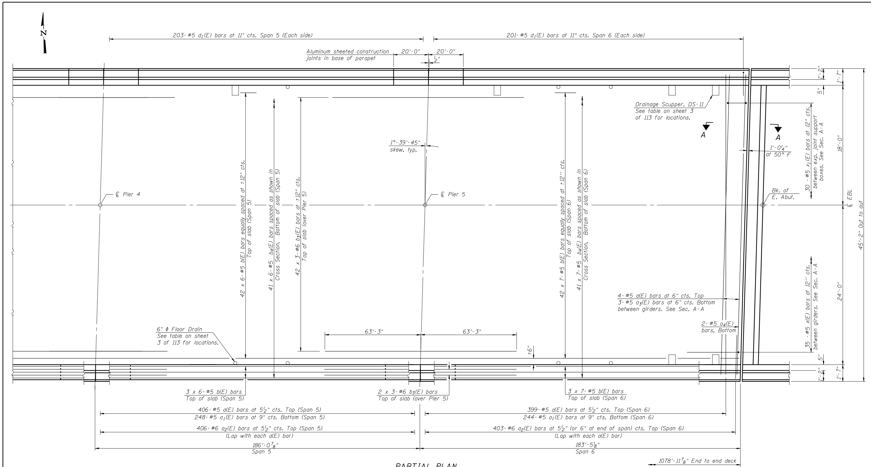
PARTIAL PLAN
