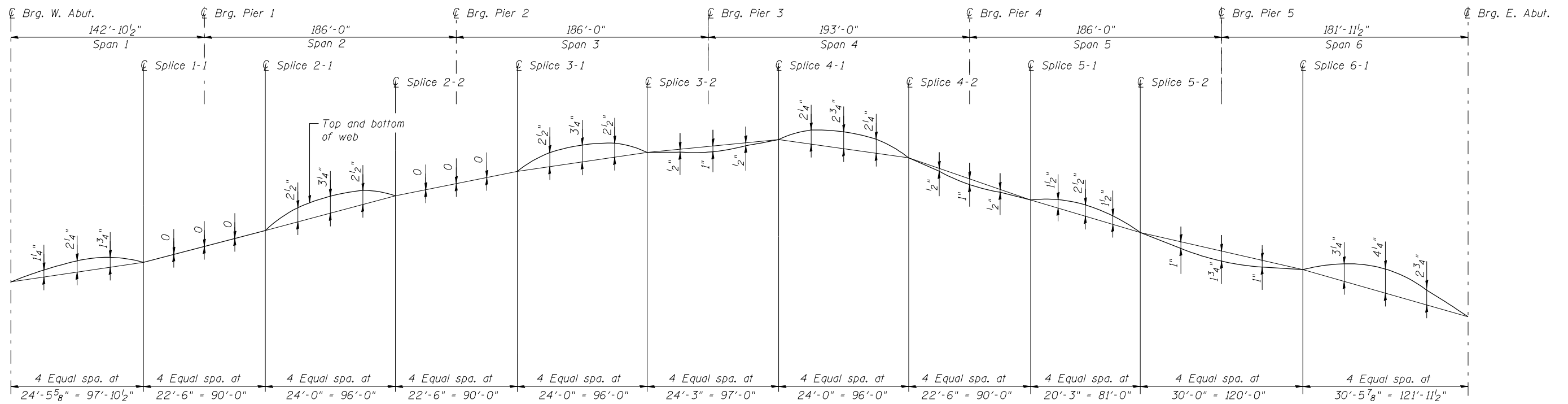
CAMBER DIAGRAM - GIRDERS 1 THRU 6
