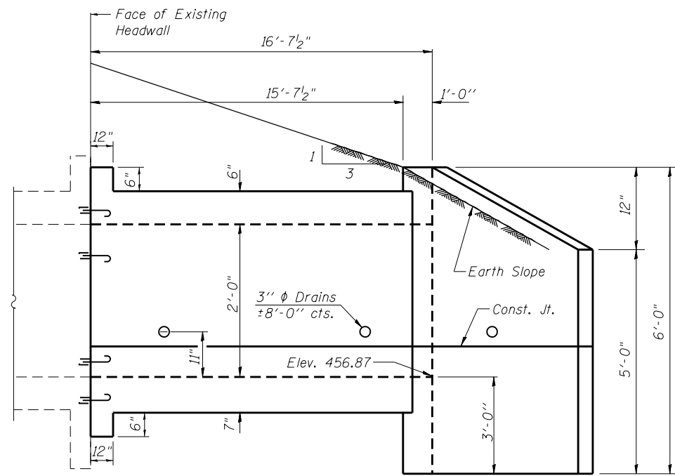
ELEVATION Dimensions at Rt. L's to \varnothing Roadway
