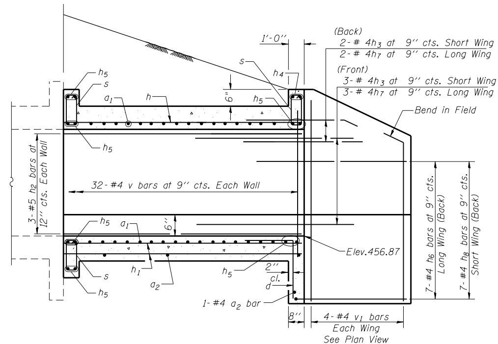
LONGITUDINAL SECTION Dimensions at Rt. L's to \varnothing Roadway
