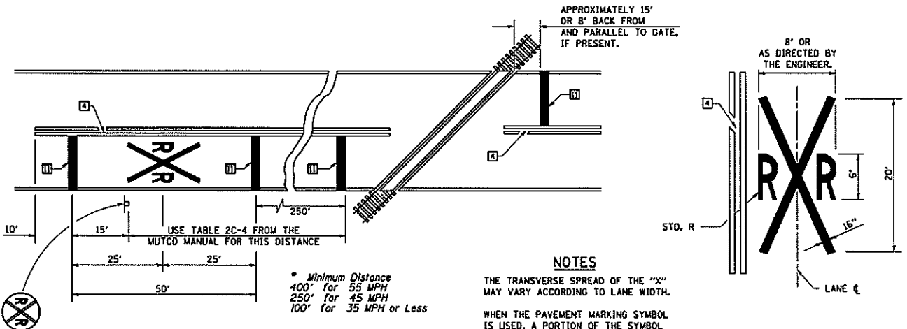
PAVEMENT MARKINGS AT RAILROAD-HIGHWAY GRADE CROSSING
