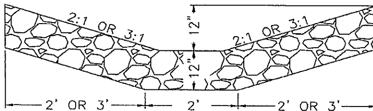
DETAIL OF AGGREGATE DITCH (SPECIAL)
