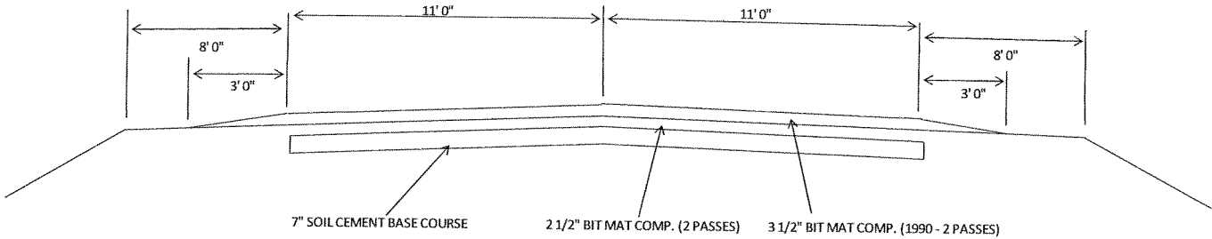
EXISTING TYPICAL SECTION E. DUBOIS ROAD STATION 41+43 to 207+17
