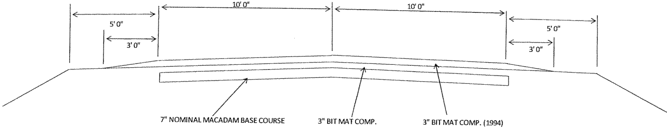
EXISTING TYPICAL SECTION E. DUBOIS ROAD STATION 0+60 to 41+57
