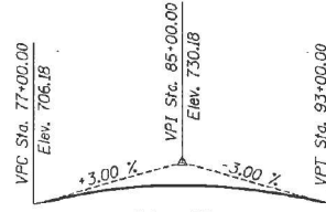
PROPOSED PROFILE GRADE F.A.P. 310
