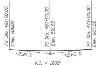
PROPOSED PROFILE GRADE N.B. & S.B. F.A.P. 310
