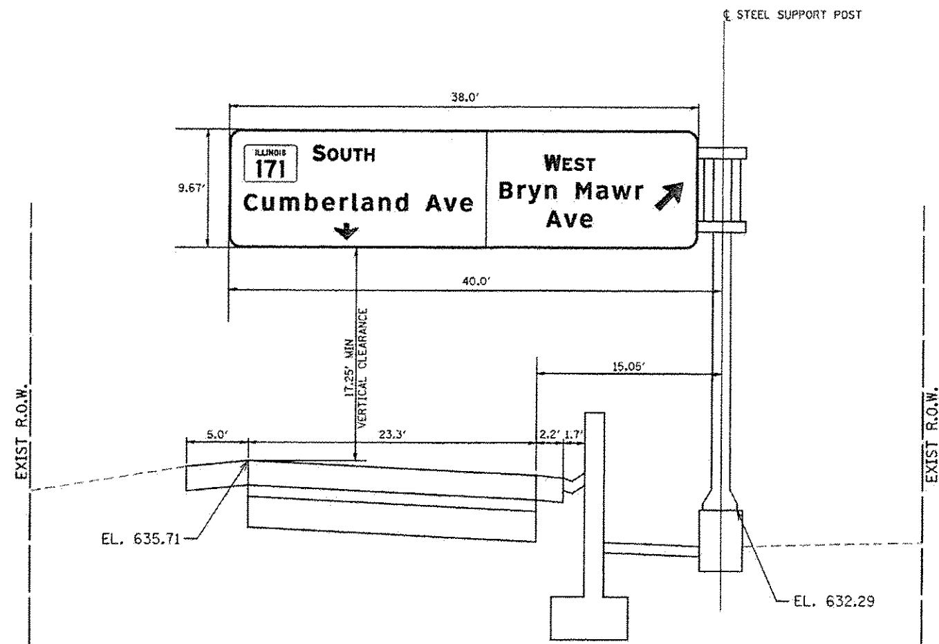
CANTILEVER OVERHEAD SIGN I-90 RAMP 6 STA. 16+35.65 (LOOKING SOUTHEAST)
