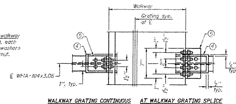
SECTION W-W
