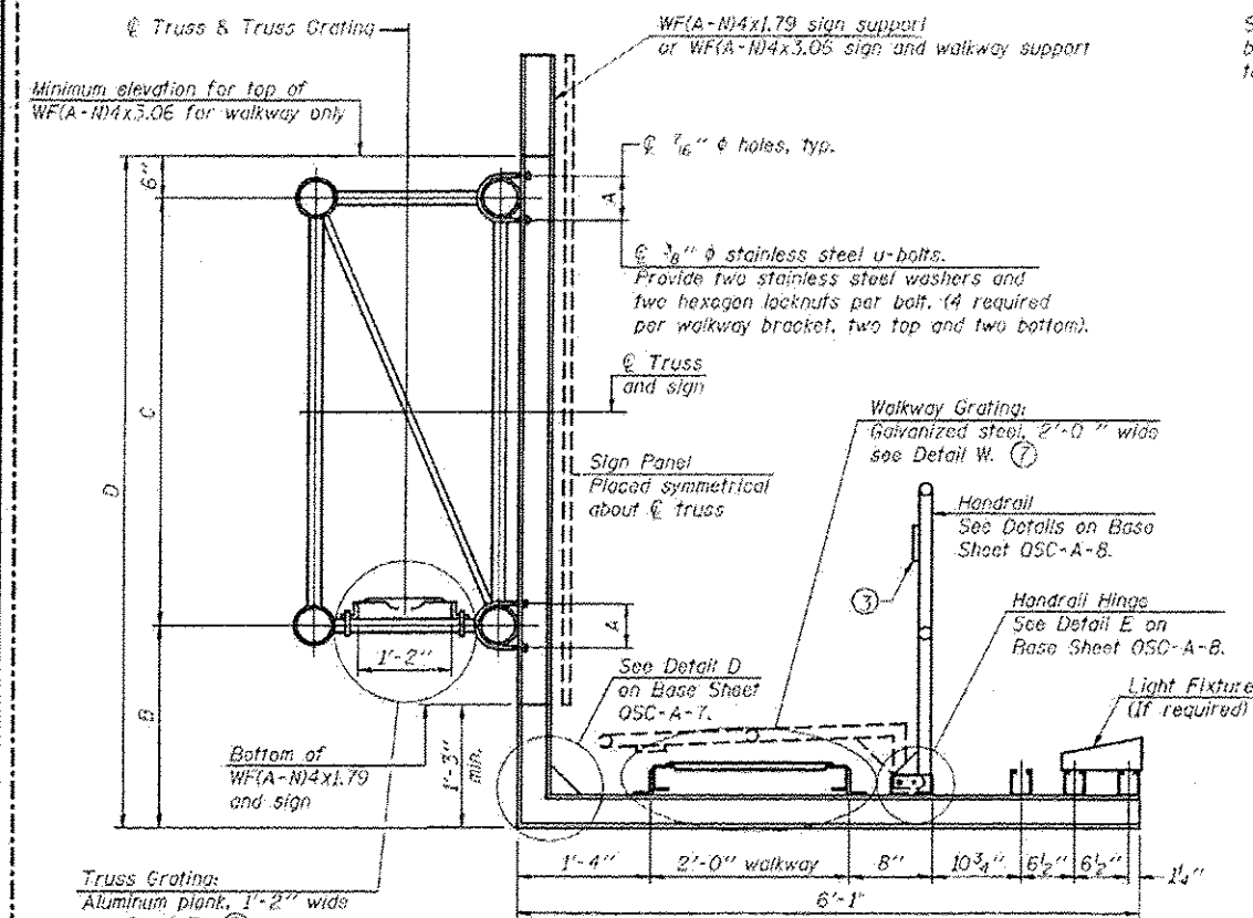
SECTION B-B
