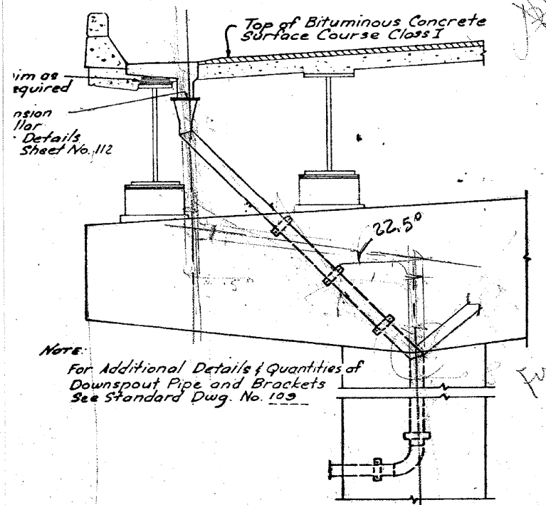
SCUPPER AT PIER
