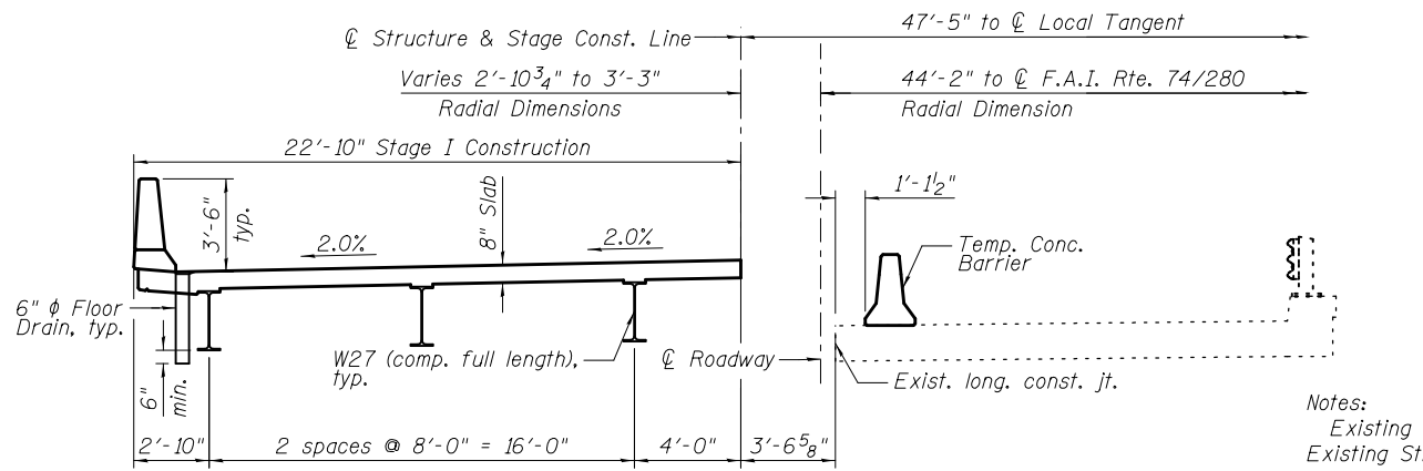
STAGE I CONSTRUCTION: SN 081-0195 (W.B.)
