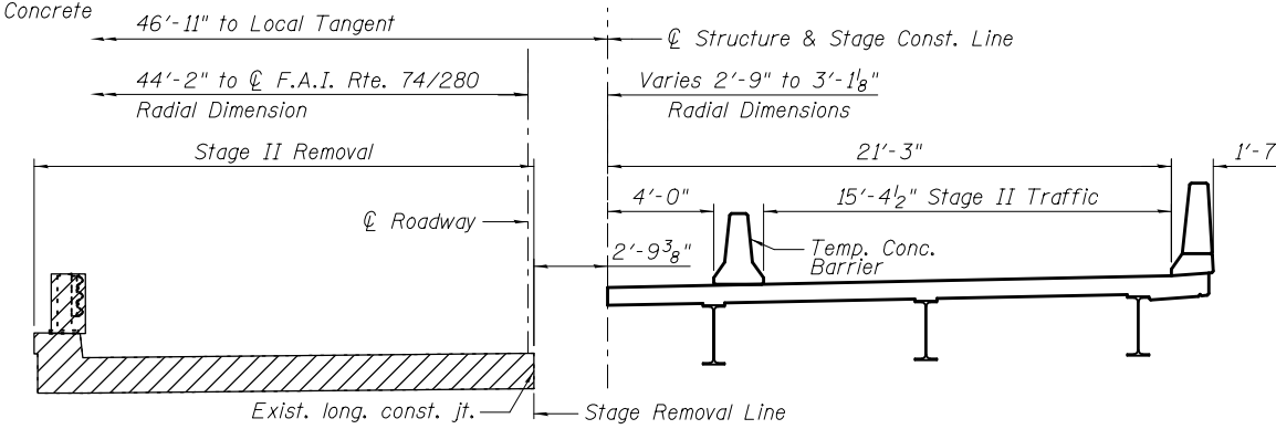
STAGE II REMOVAL: SN 081-0194 (E.B.)
