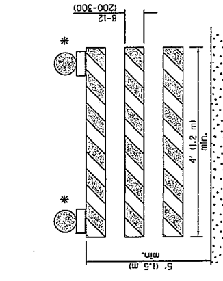
FLEXIBLE DELINEATOR
