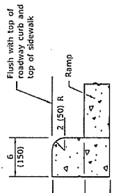
SIDE CURB DETAIL
