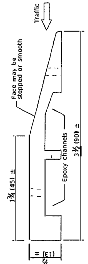
TEMPORARY RUMBLE STRIPS
