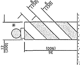
VERTICAL BARRICADE
