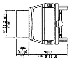
TYPE A ARROW BOARD ROOF MOUNTED
