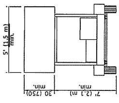
TYPE B ARROW BOARD ROOF OR TRAILER MOUNTED
