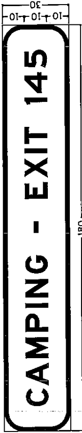
G5, F5, L5, C5 MAINLINE SIGN
