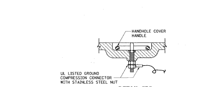
DETAIL "B"
