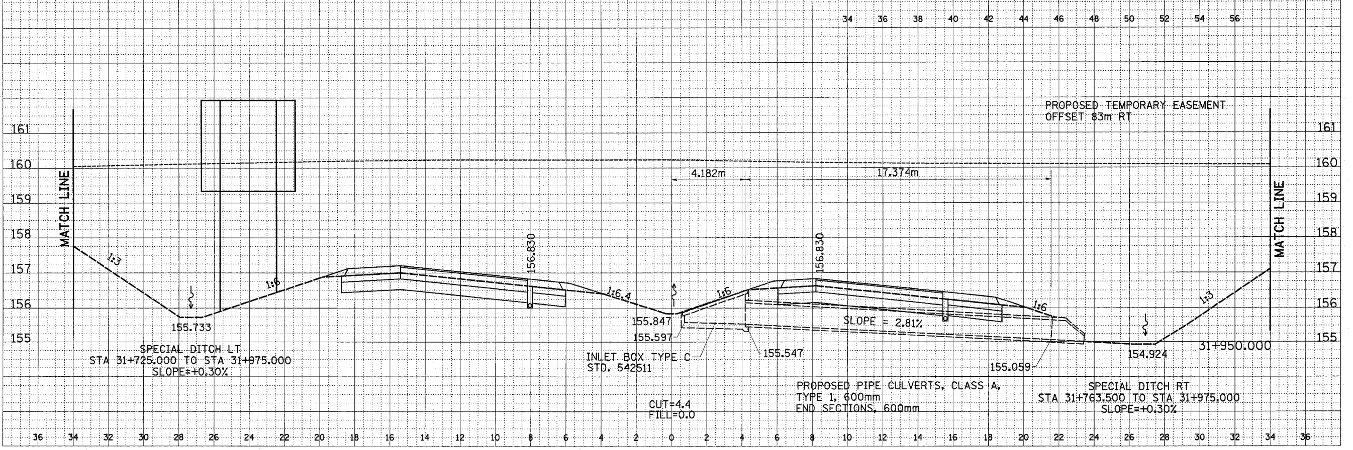
CROSS SECTION, FAP ROUTE 310, STA 31+950.000
