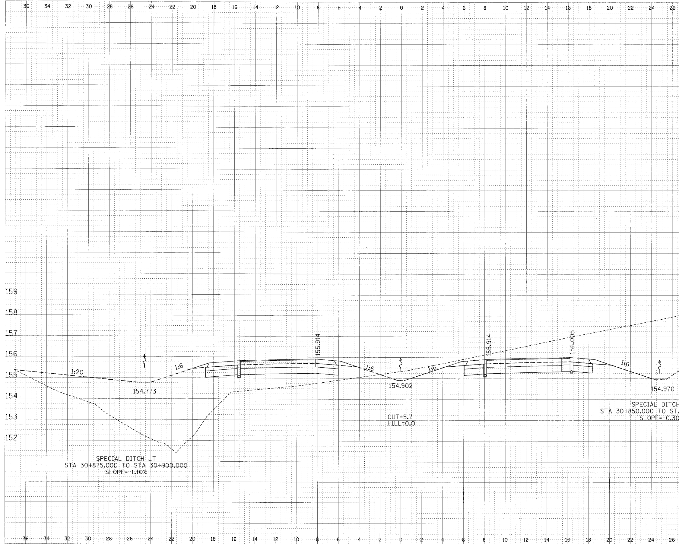
CROSS SECTION, FAP ROUTE 310, STA 30+875.000
