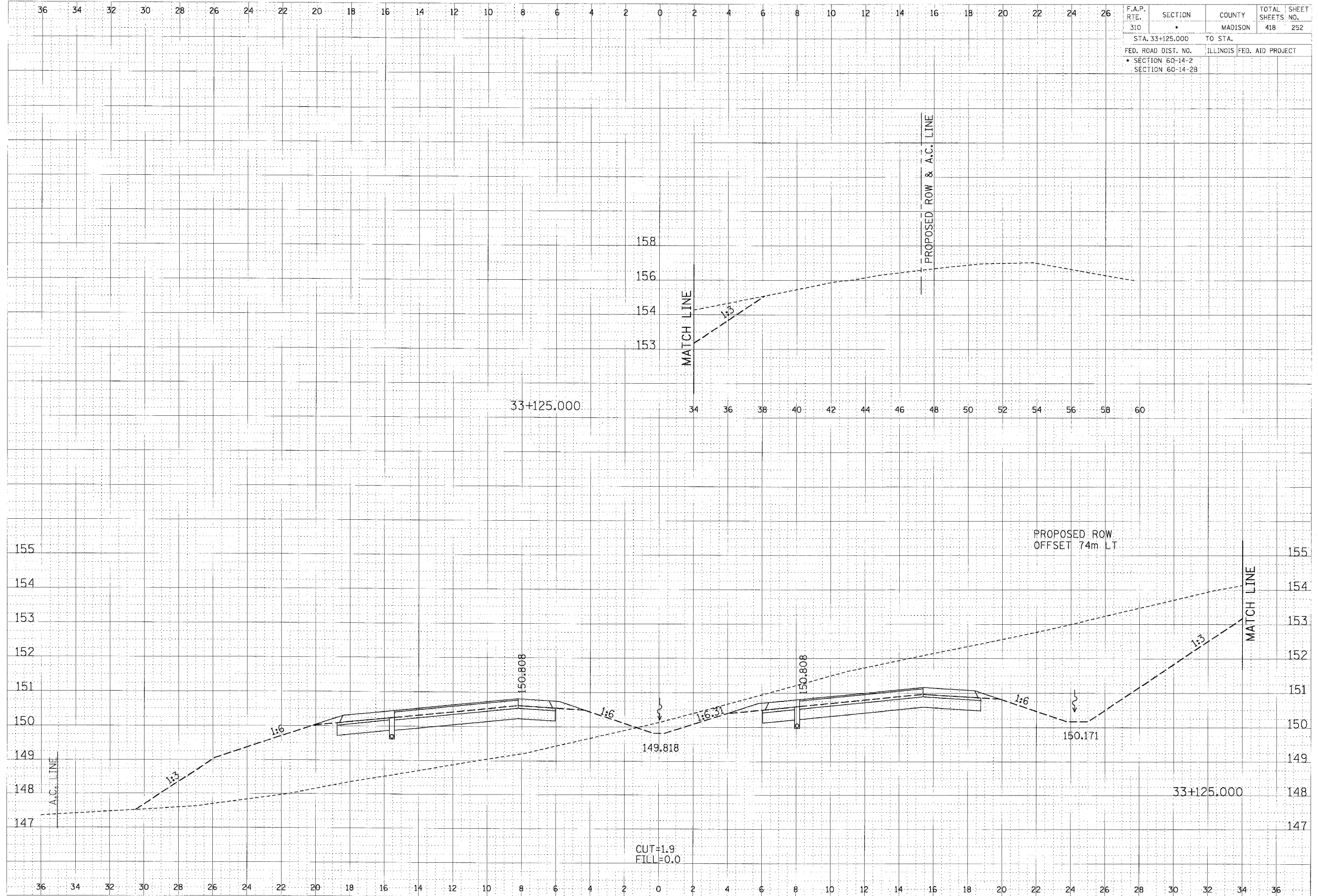
CROSS SECTION, FAP ROUTE 310, STA 33+125.000
