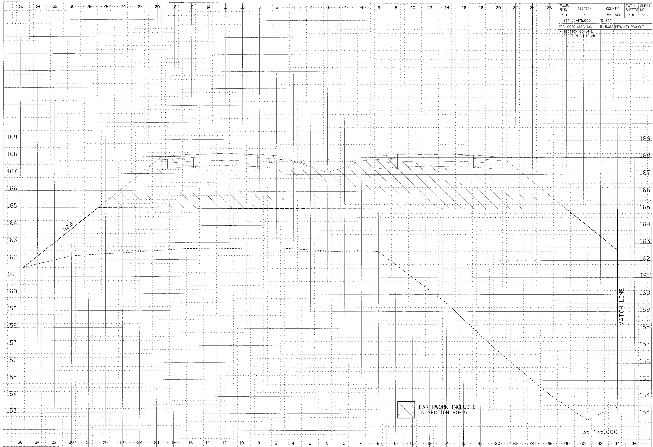
CROSS SECTION, FAP ROUTE 310, STA 35+175.000
