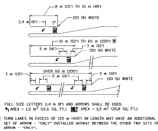
TYPICAL LEFT (OR RIGHT) TURN LANE
