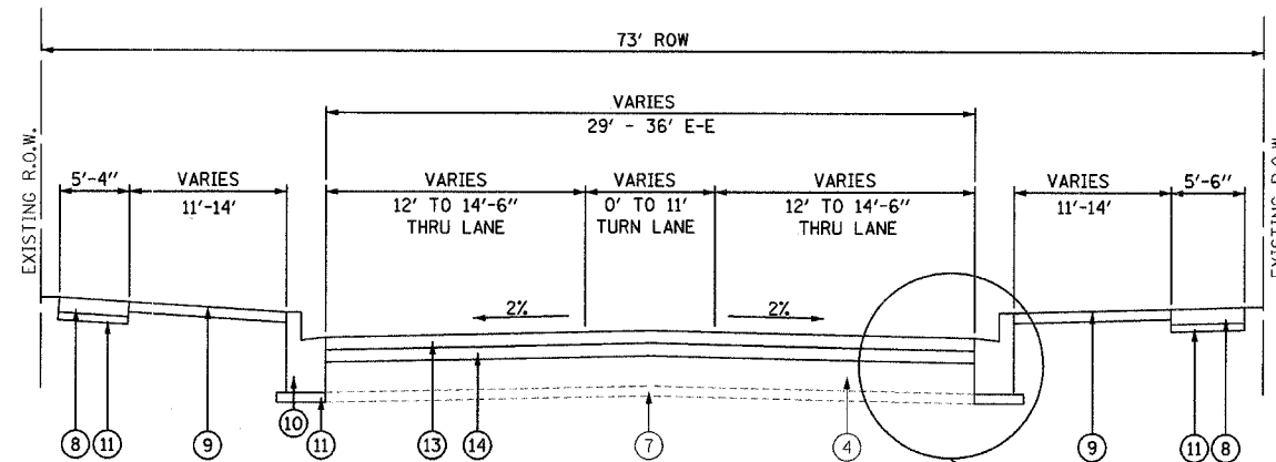
PROPOSED TYPICAL CROSS SECTION STA. 100+49 TO STA. 101+44
