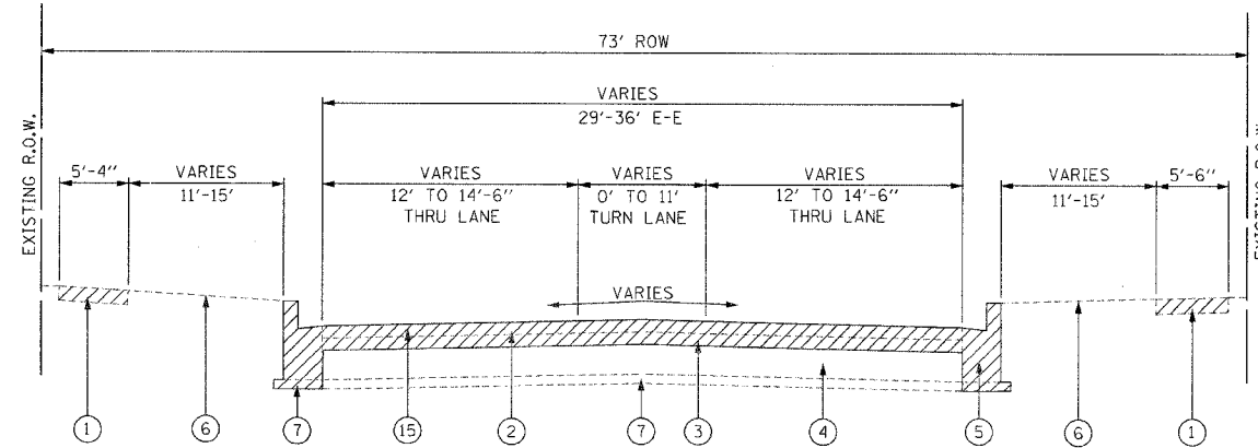
EXISTING TYPICAL CROSS SECTION STA. 100+49 TO STA. 101+44
