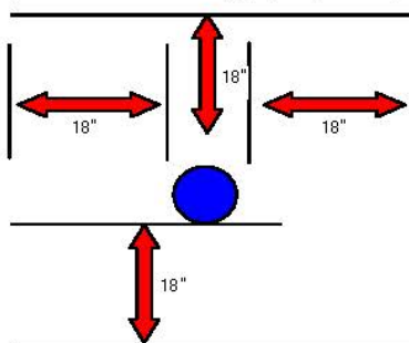
Figure 1 – Horizontal and Vertical Offsets
