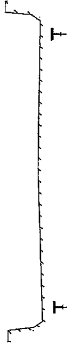
CROSS SECTION WITH PARAPET
