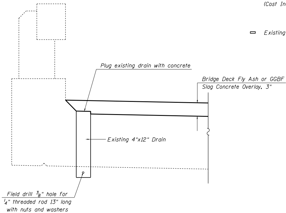
DRAINS TO BE PLUGGED DETAIL
