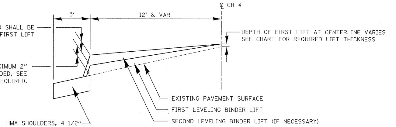
TYPICAL CROSS SECTION OF LEVELING BINDER LIFT CONSTRUCTION
