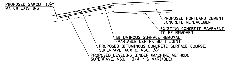
SECTION A-A EXISTING BITUMINOUS SURFACE
