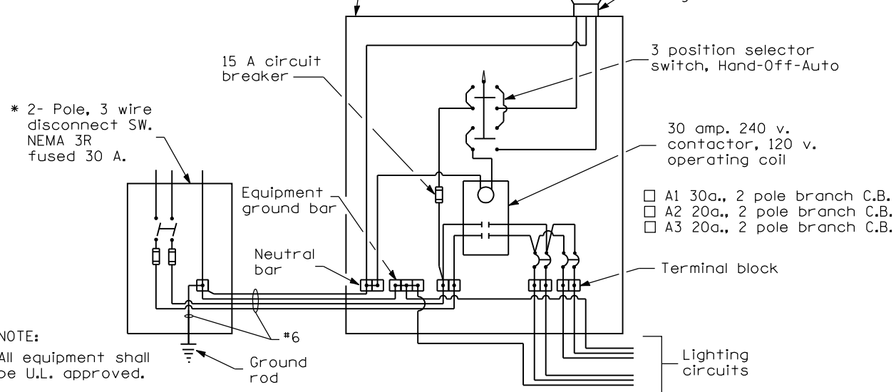
WIRING DIAGRAM
