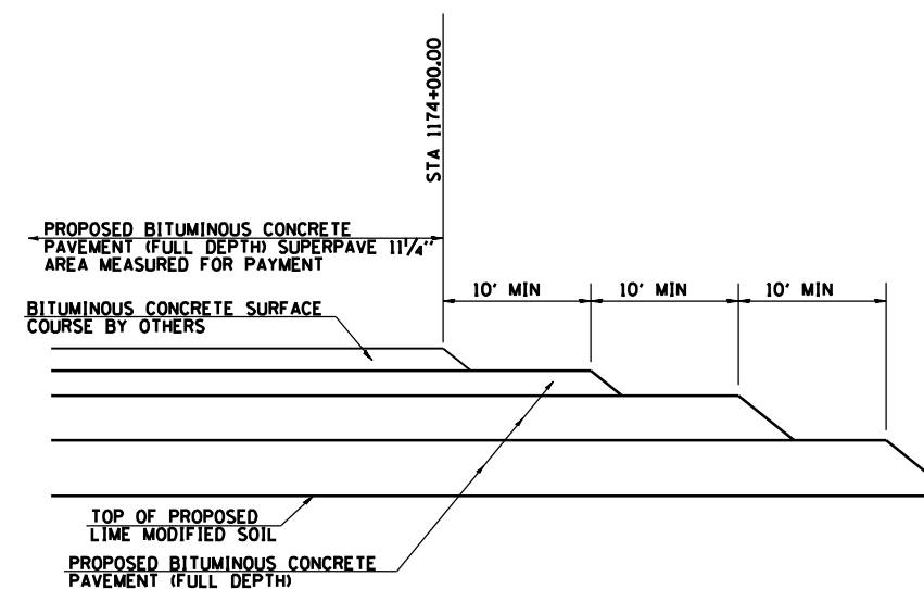
DETAIL OF TERMINATION OF PROPOSED FULL-DEPTH BITUMINOUS CONCRETE PAVEMENT AT EAST END
