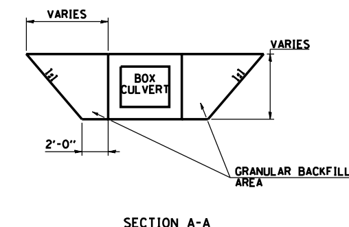
GRANULAR CULVERT BACKFILL
