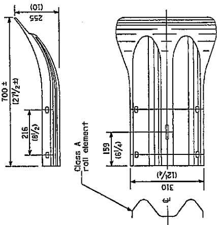
END SECTION
