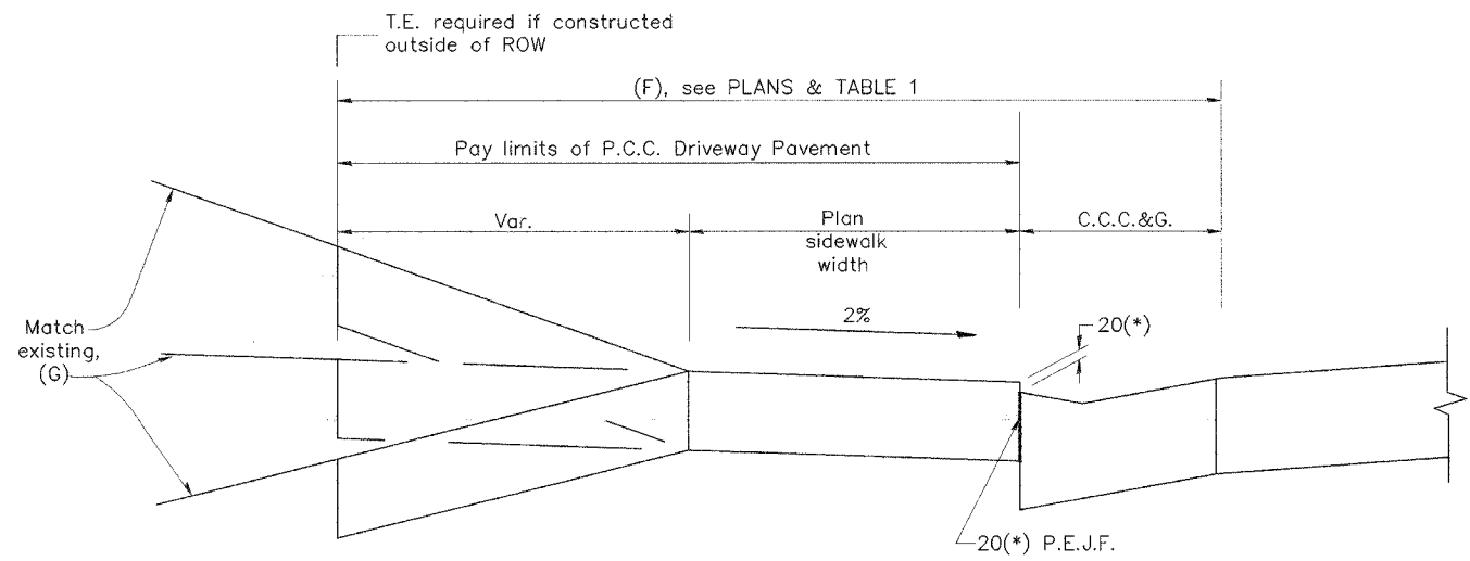
SECTION B-B
