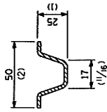
SECTION E-E 1.67 kg/m Steel - (112 lbs./ft.)
