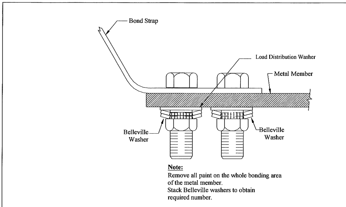
Figure I. Order of Assembly for Bolted Connections
