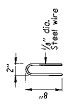
STAPLE DETAIL
