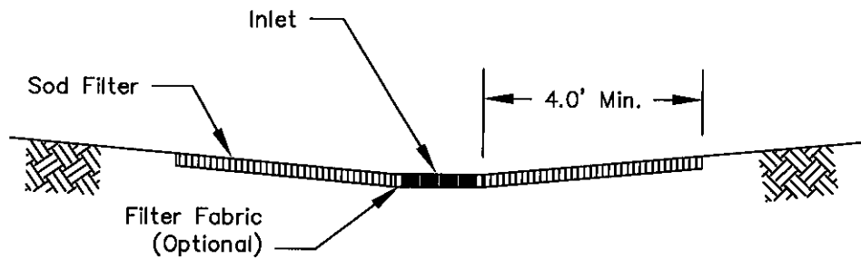
SECTION
