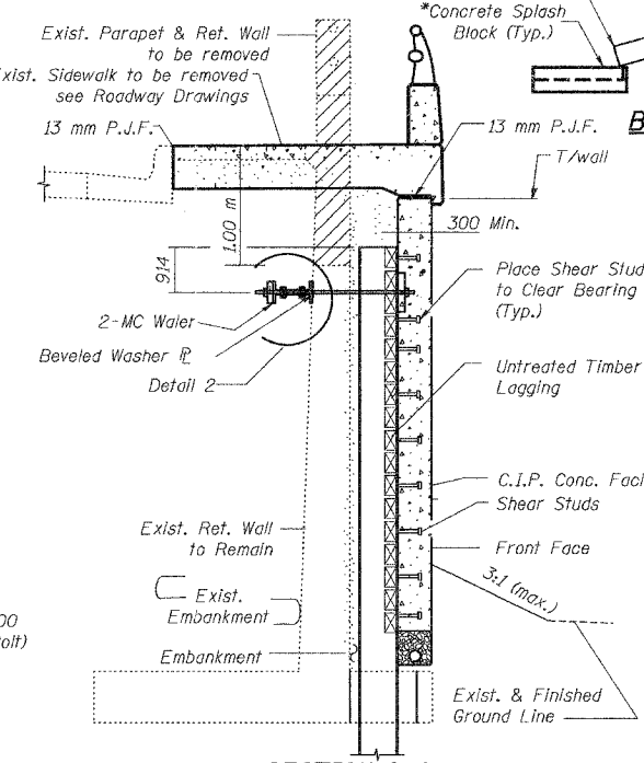
SECTION C-C (NEAR EAST CORNER OF NORTH ABUTMENT)
