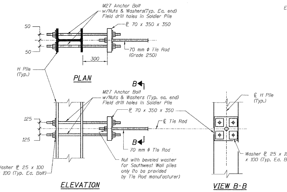
DETAIL 1
