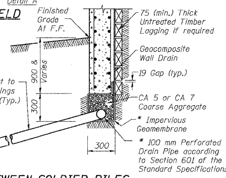
PIPE UNDERDRAIN DETAILS
