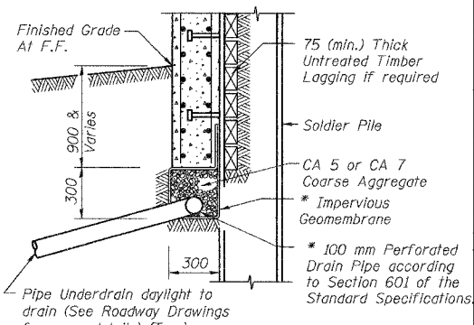
PIPE UNDERDRAIN DETAILS
