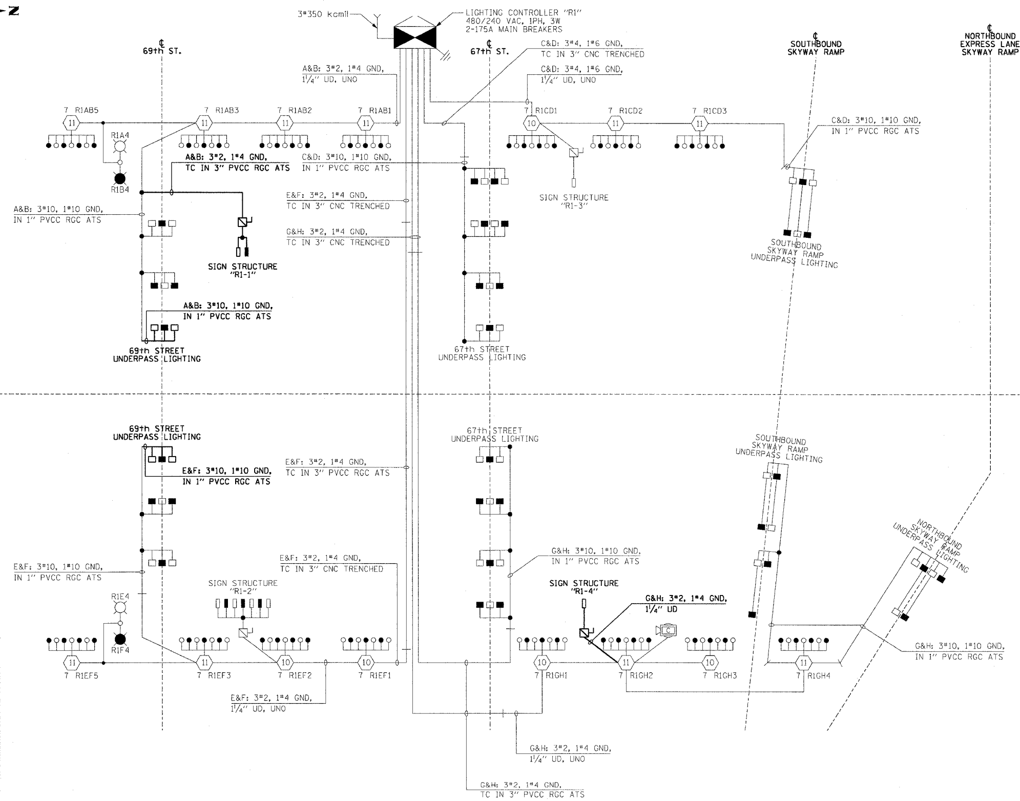
SINGLE LINE DIAGRAM LIGHTING CONTROLLER "R1" NOT TO SCALE
