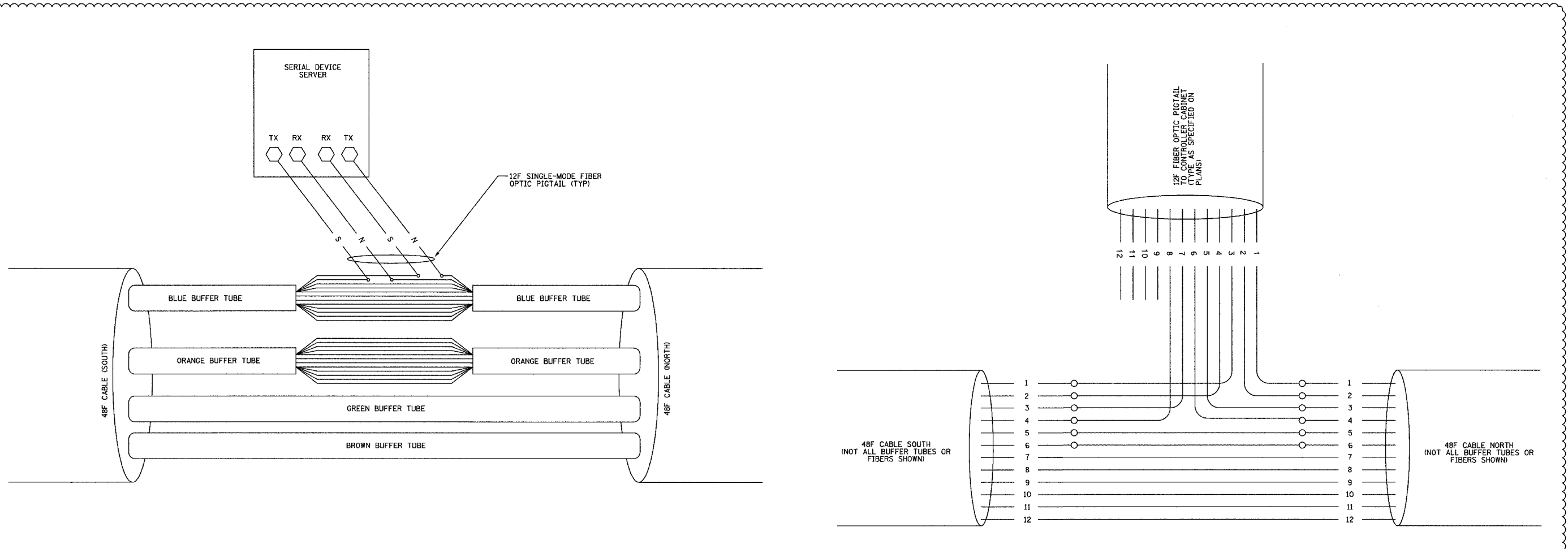
PHYSICAL SPLICE DETAILS (TYP) NOT TO SCALE
