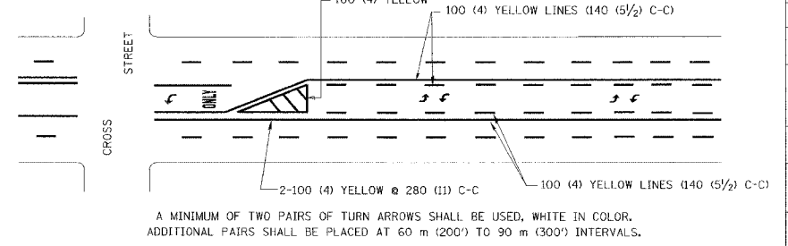
TYPICAL PAINTED MEDIAN MARKING
