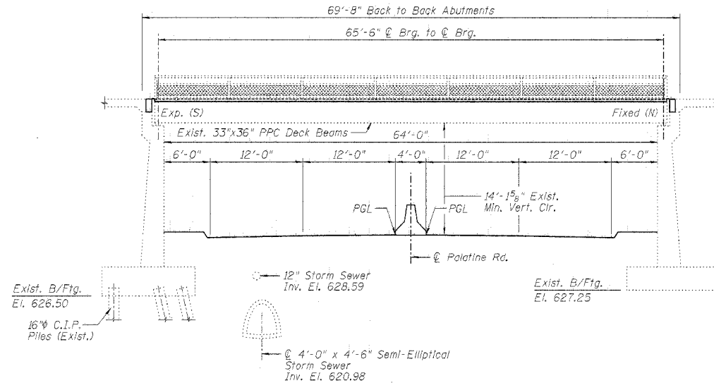
ELEVATION (Looking West)
