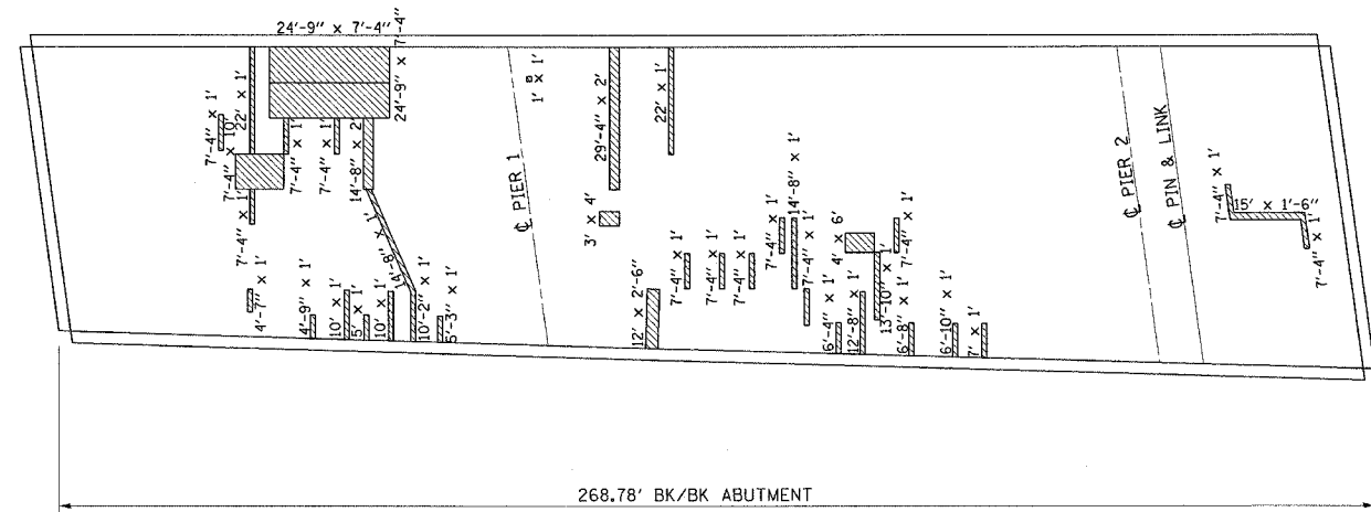
PLAN DECK REPAIR
